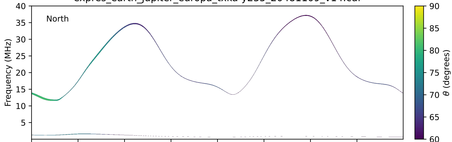
expres_earth_jupiter_europa_txka-y235_20481109_v14.cdf
