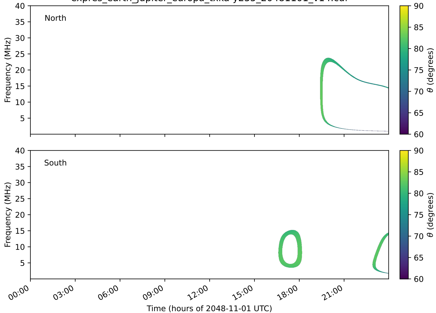
expres_earth_jupiter_europa_txka-y235_20481101_v14.cdf
