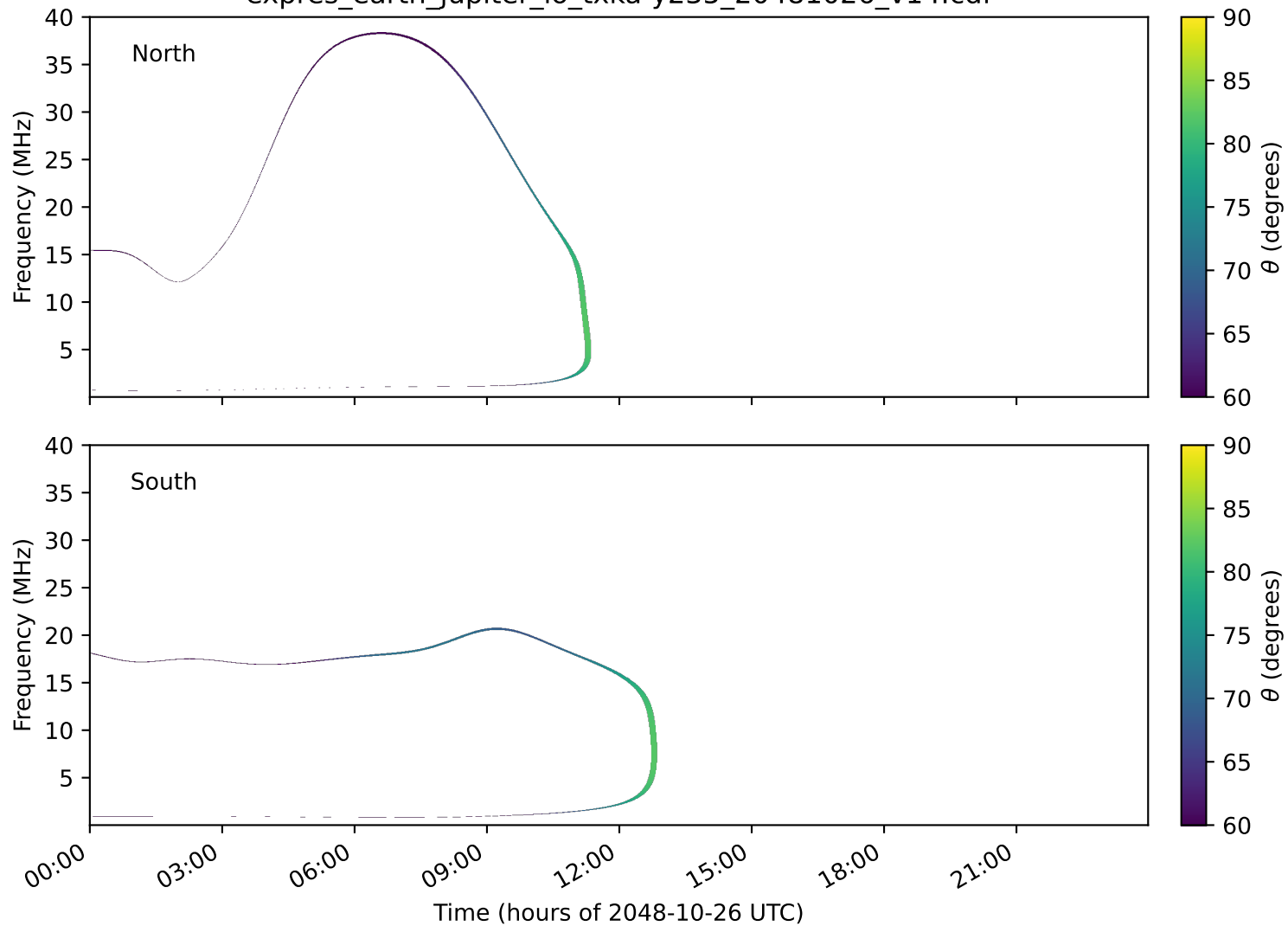
expres_earth_jupiter_io_txka-y235_20481026_v14.cdf
