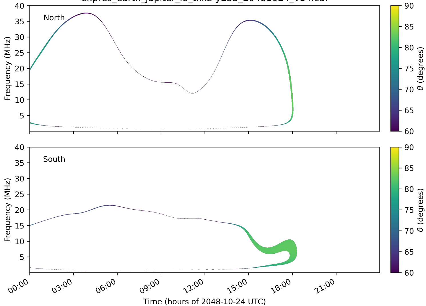
expres_earth_jupiter_io_txka-y235_20481024_v14.cdf
