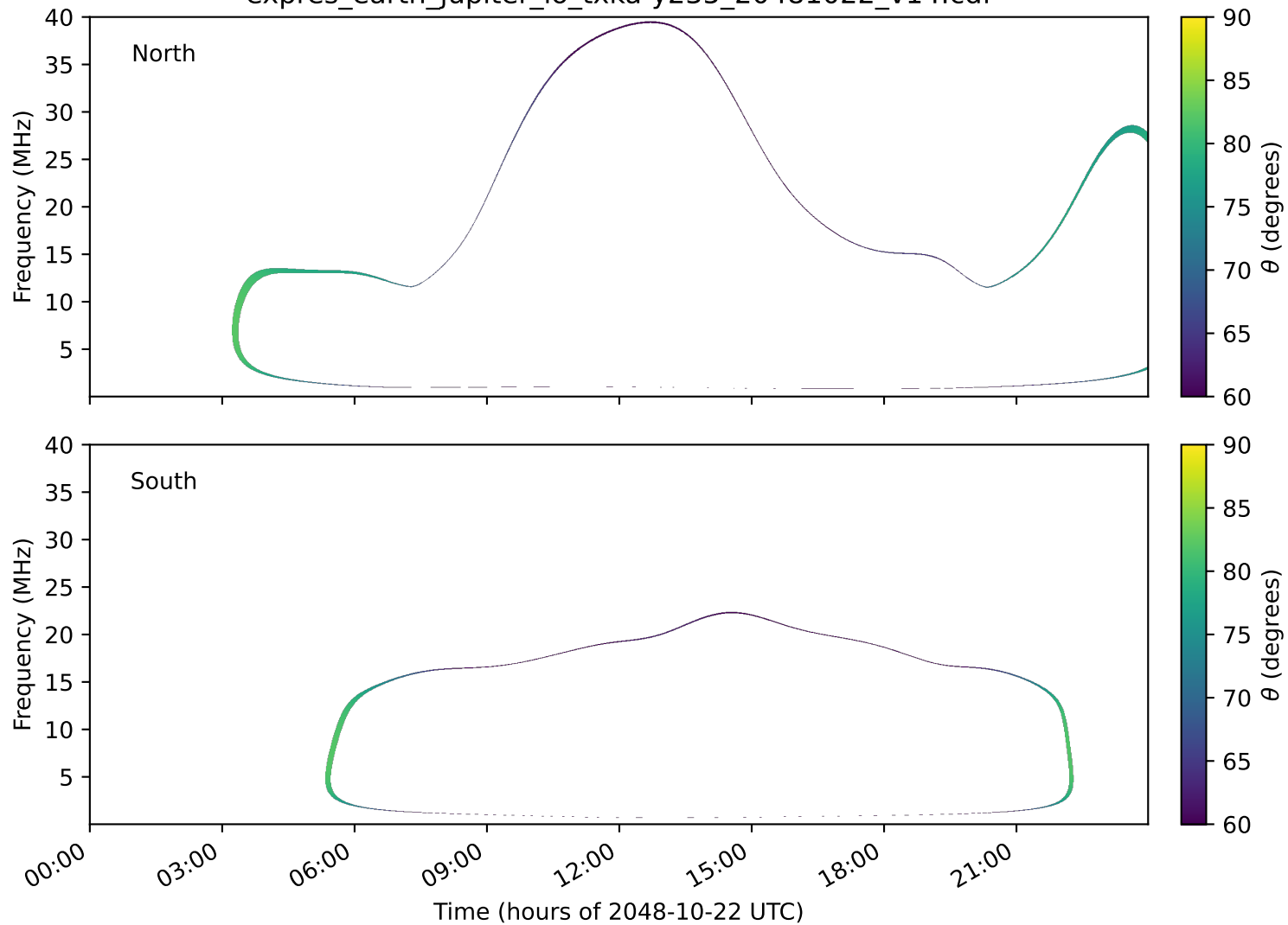
expres_earth_jupiter_io_txka-y235_20481022_v14.cdf
