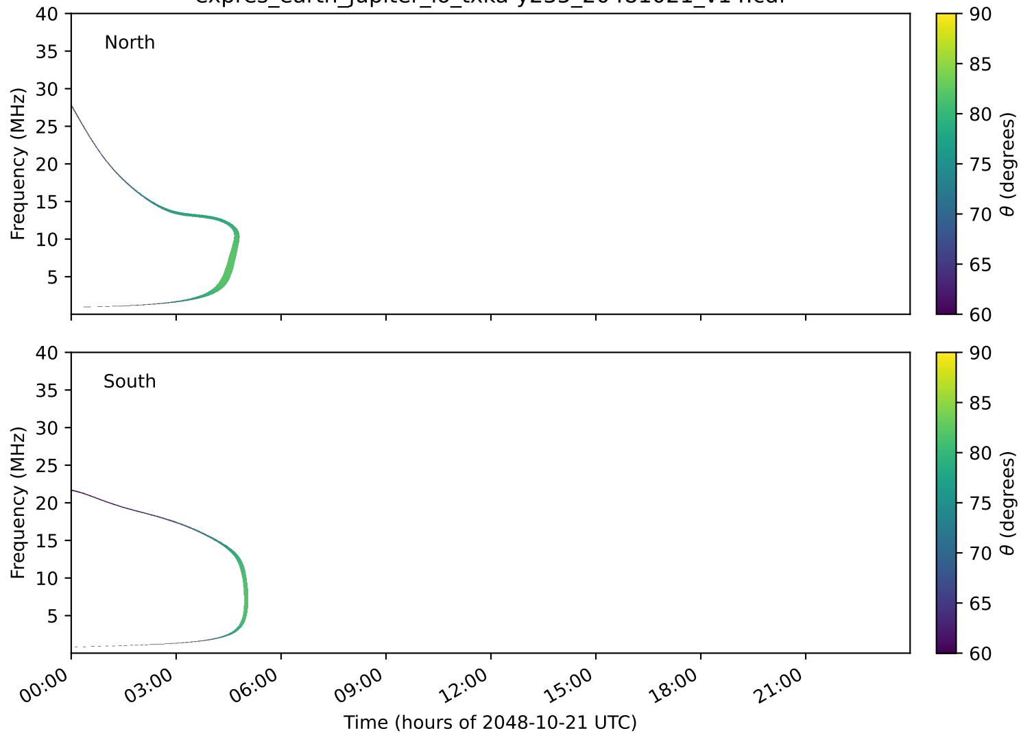
expres_earth_jupiter_io_txka-y235_20481021_v14.cdf
