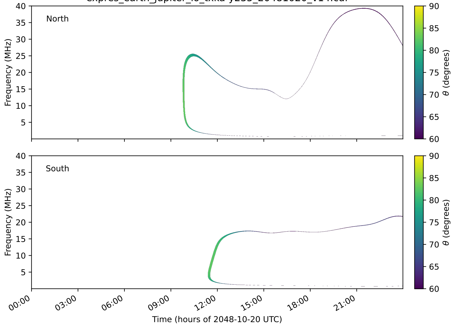
expres_earth_jupiter_io_txka-y235_20481020_v14.cdf
