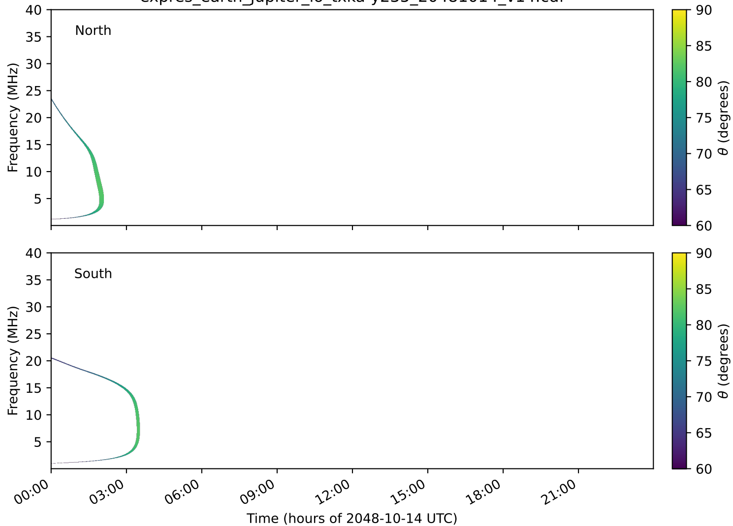
expres_earth_jupiter_io_txka-y235_20481014_v14.cdf
