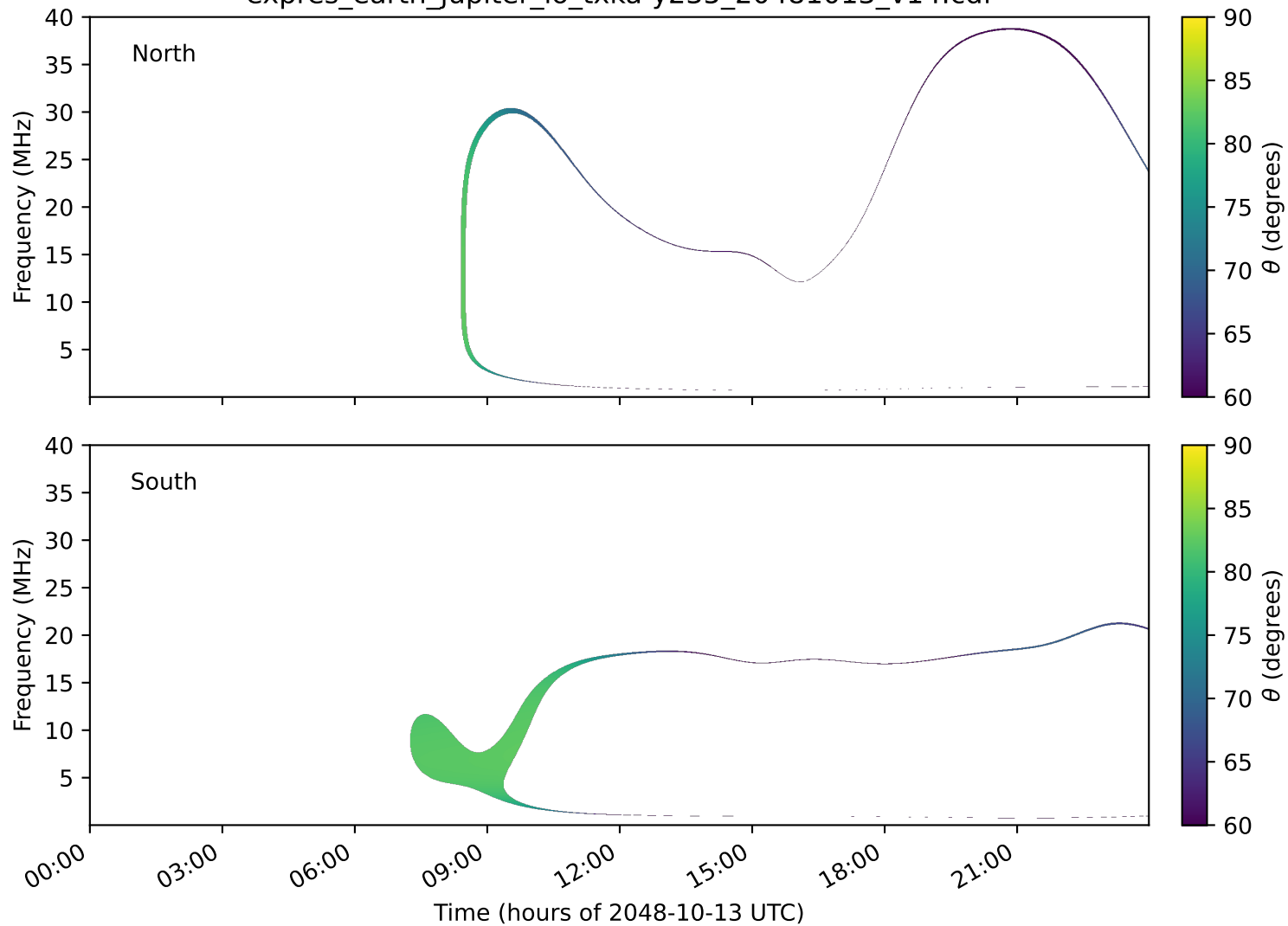
expres_earth_jupiter_io_txka-y235_20481013_v14.cdf
