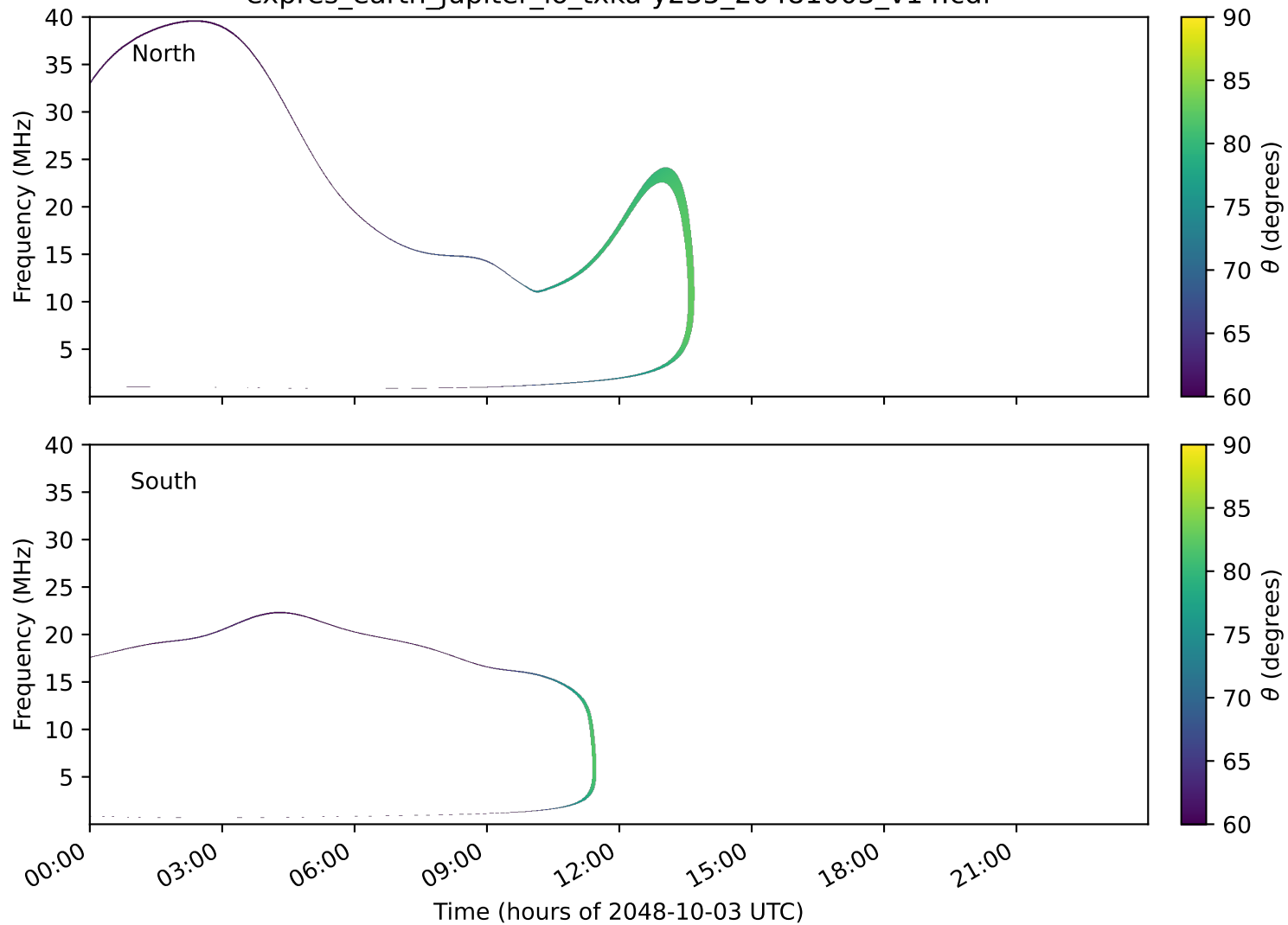
expres_earth_jupiter_io_txka-y235_20481003_v14.cdf
