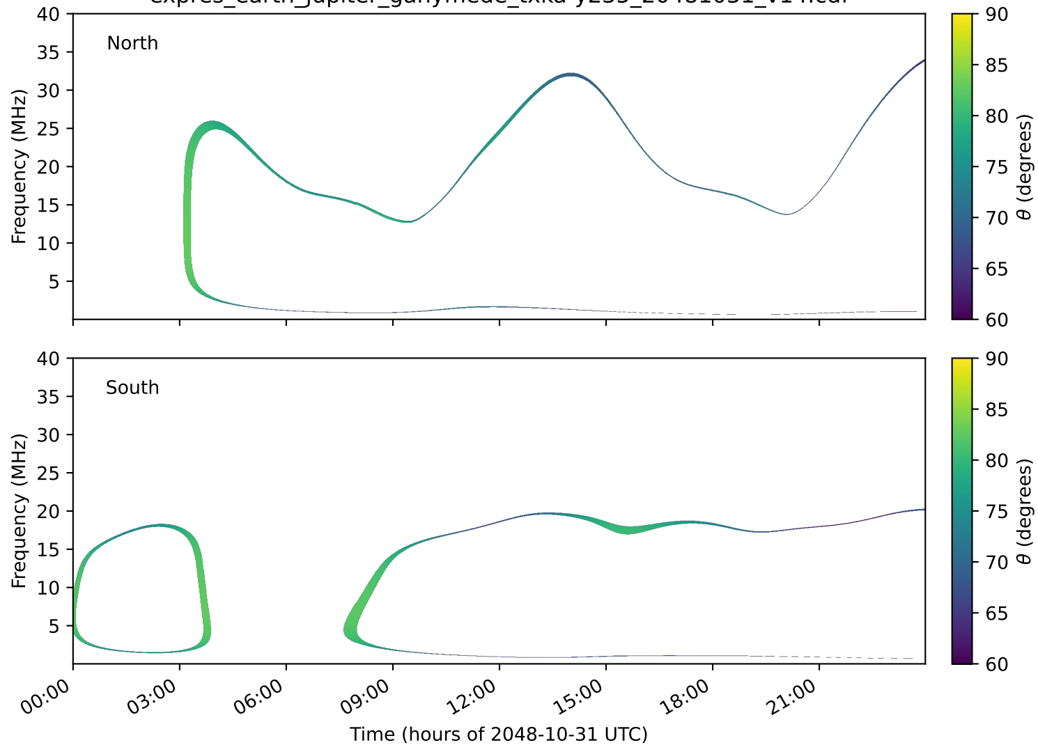
expres_earth_jupiter_ganymede_txka-y235_20481031_v14.cdf
