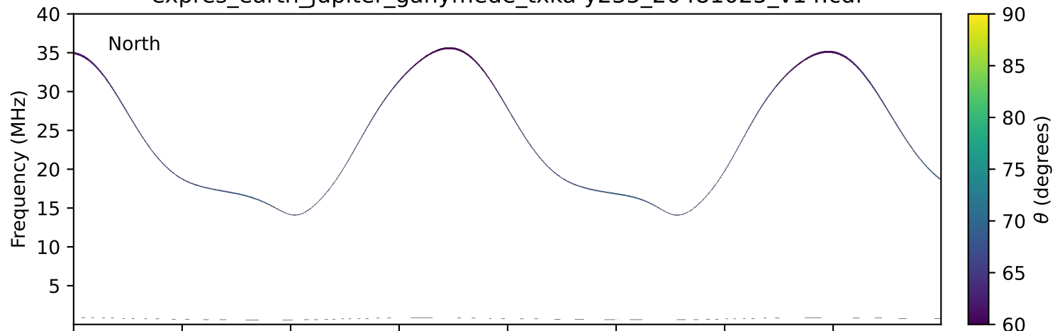
expres_earth_jupiter_ganymede_txka-y235_20481025_v14.cdf
