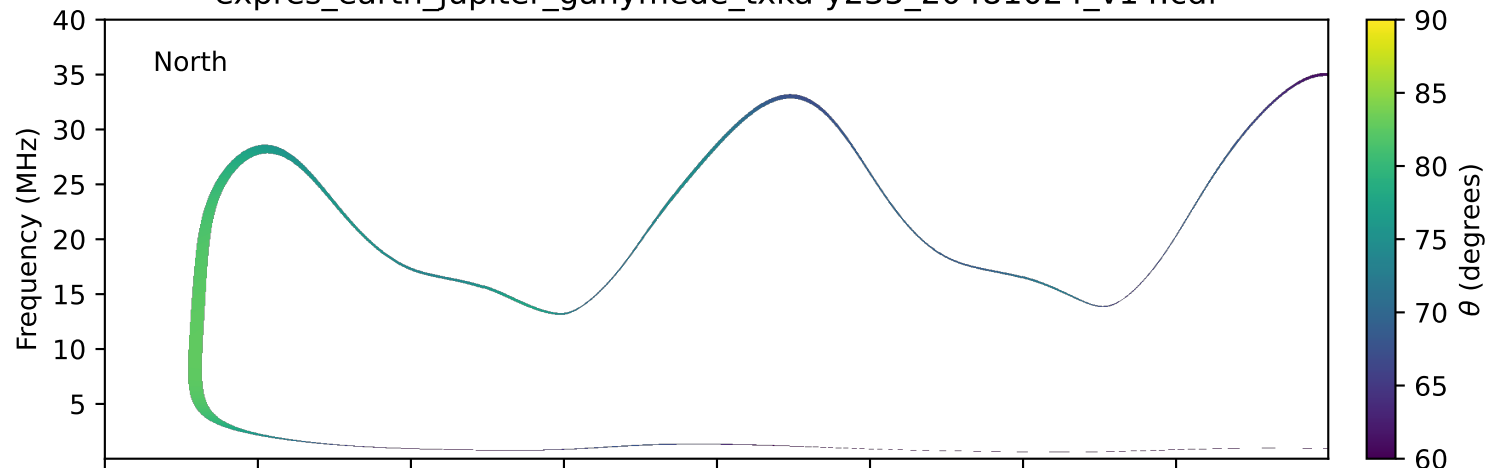
expres_earth_jupiter_ganymede_txka-y235_20481024_v14.cdf
