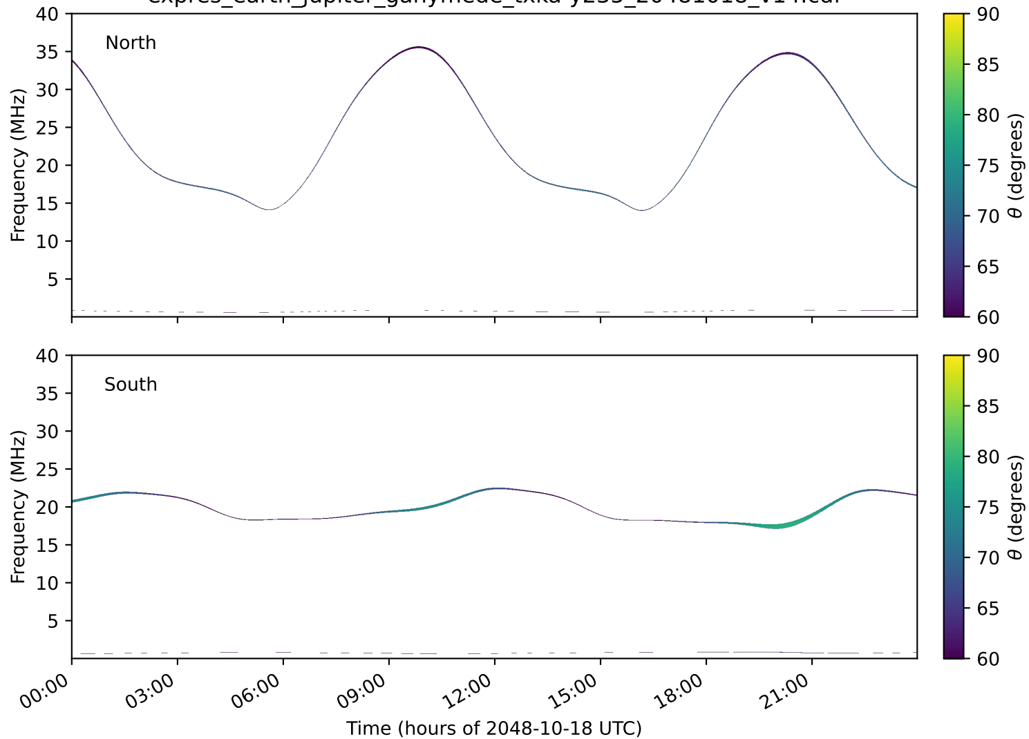
expres_earth_jupiter_ganymede_txka-y235_20481018_v14.cdf
