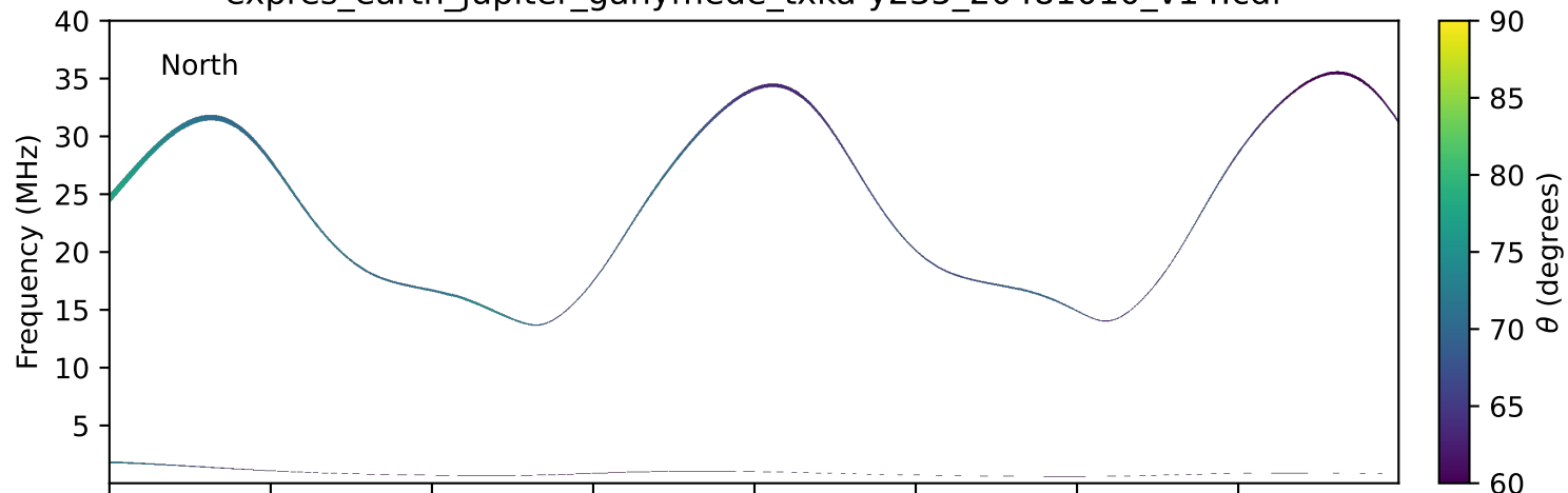
expres_earth_jupiter_ganymede_txka-y235_20481010_v14.cdf
