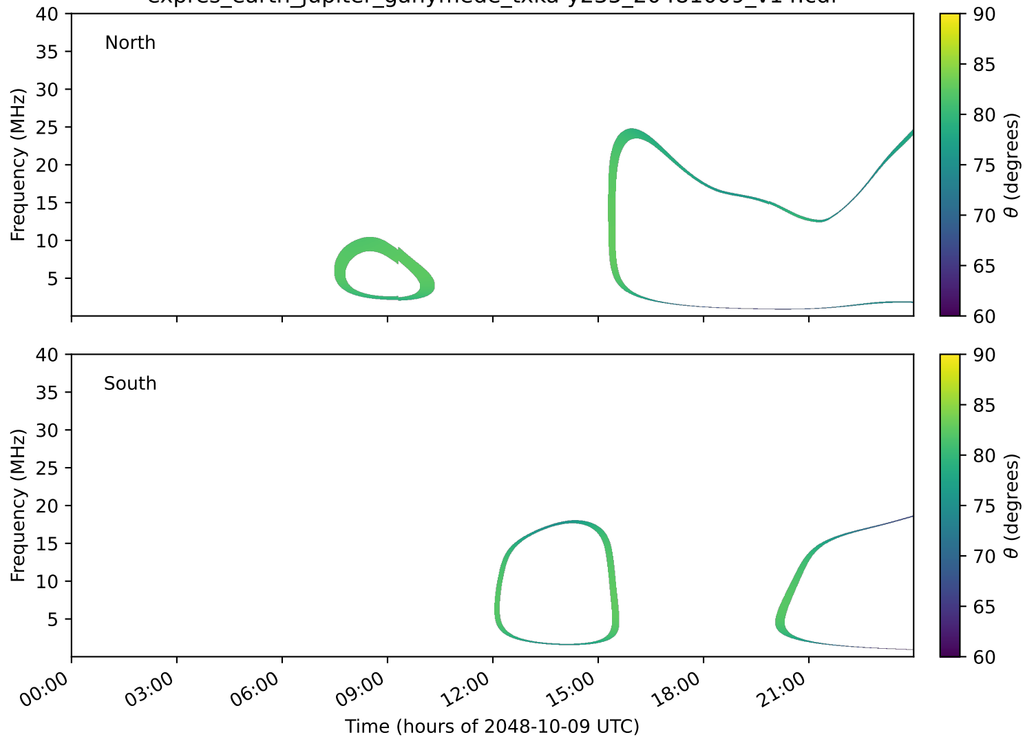
expres_earth_jupiter_ganymede_txka-y235_20481009_v14.cdf
