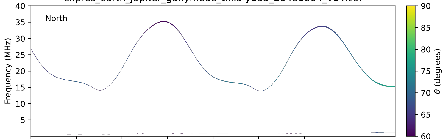
expres_earth_jupiter_ganymede_txka-y235_20481004_v14.cdf
