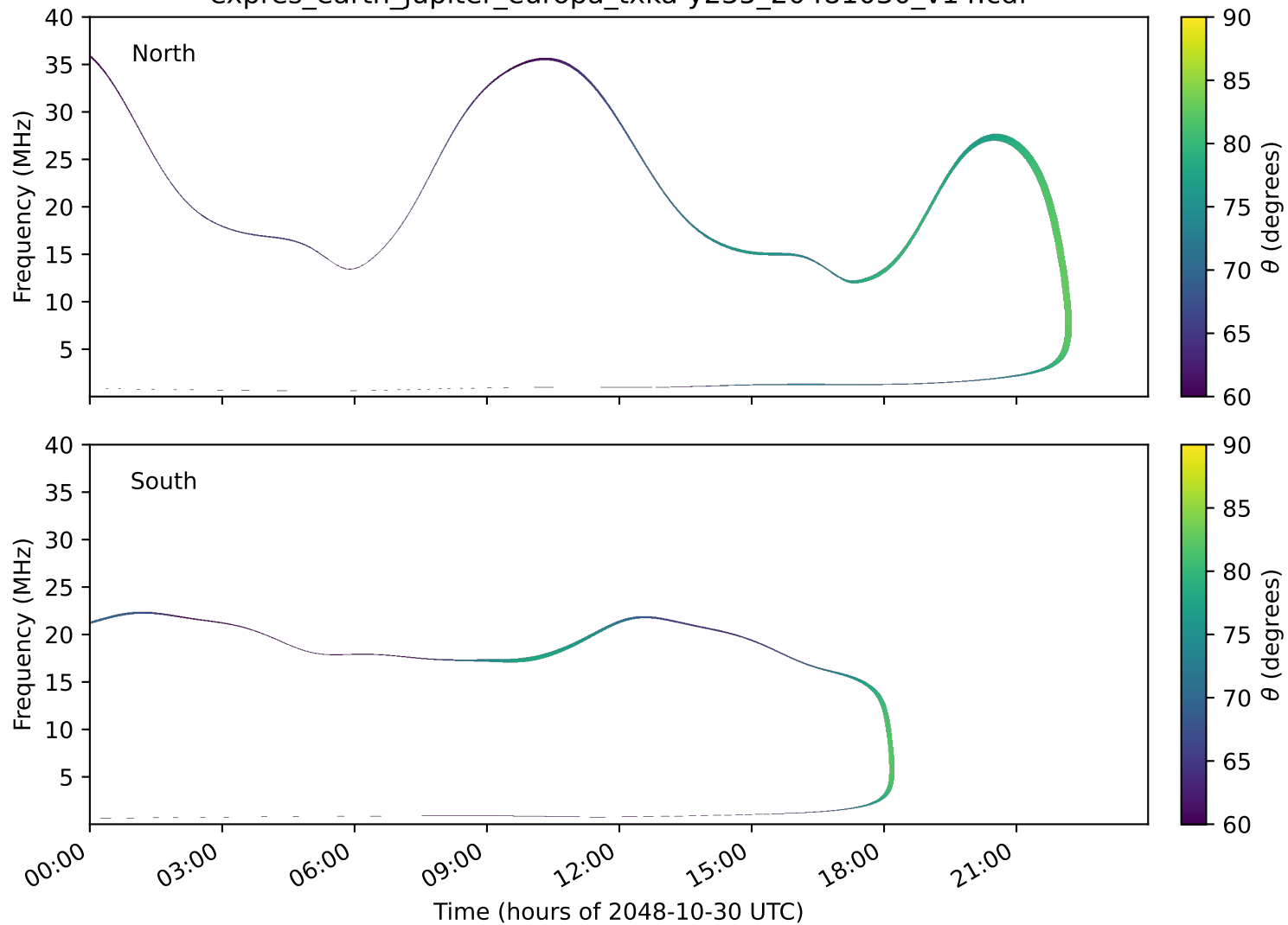
expres_earth_jupiter_europa_txka-y235_20481030_v14.cdf
