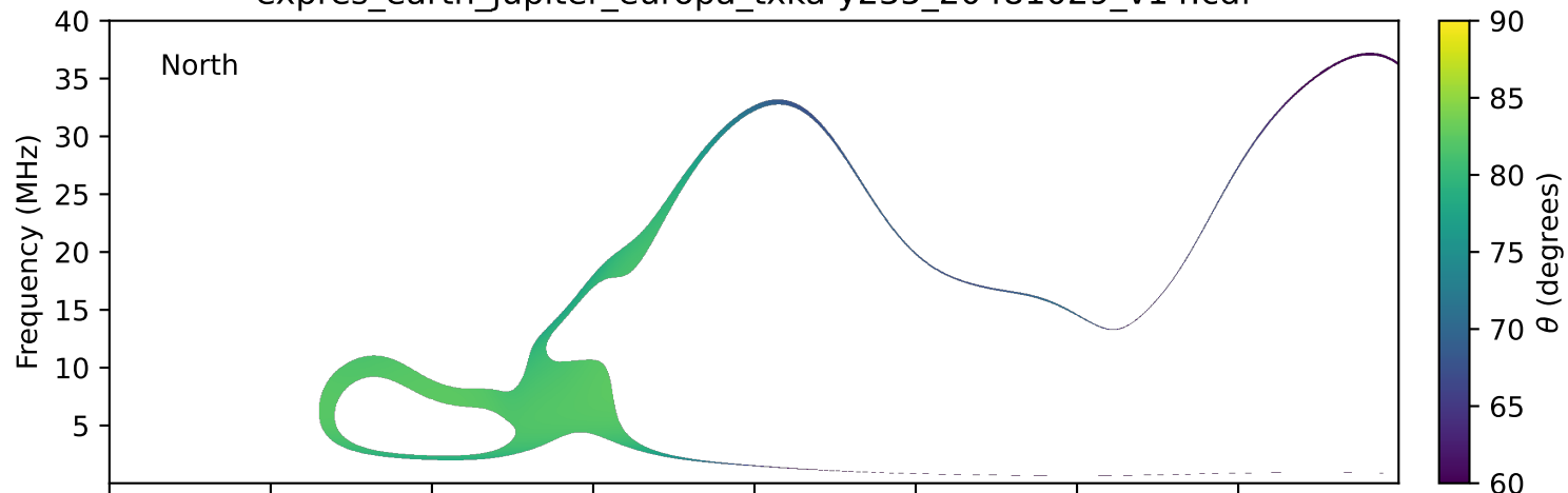
expres_earth_jupiter_europa_txka-y235_20481029_v14.cdf
