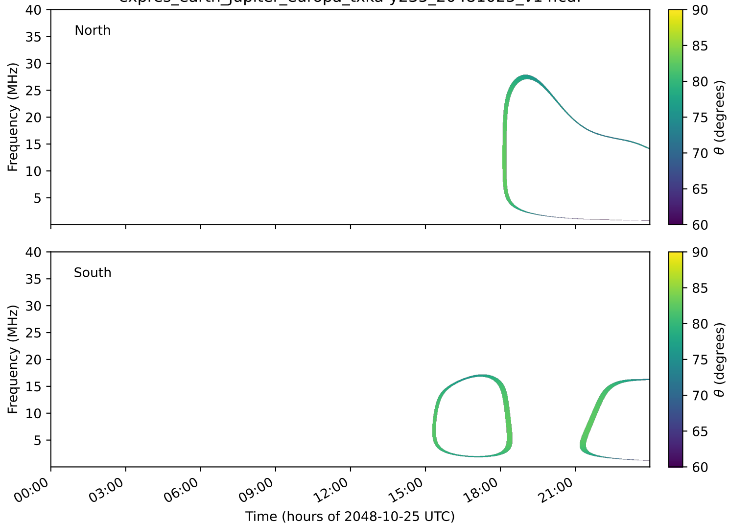
expres_earth_jupiter_europa_txka-y235_20481025_v14.cdf
