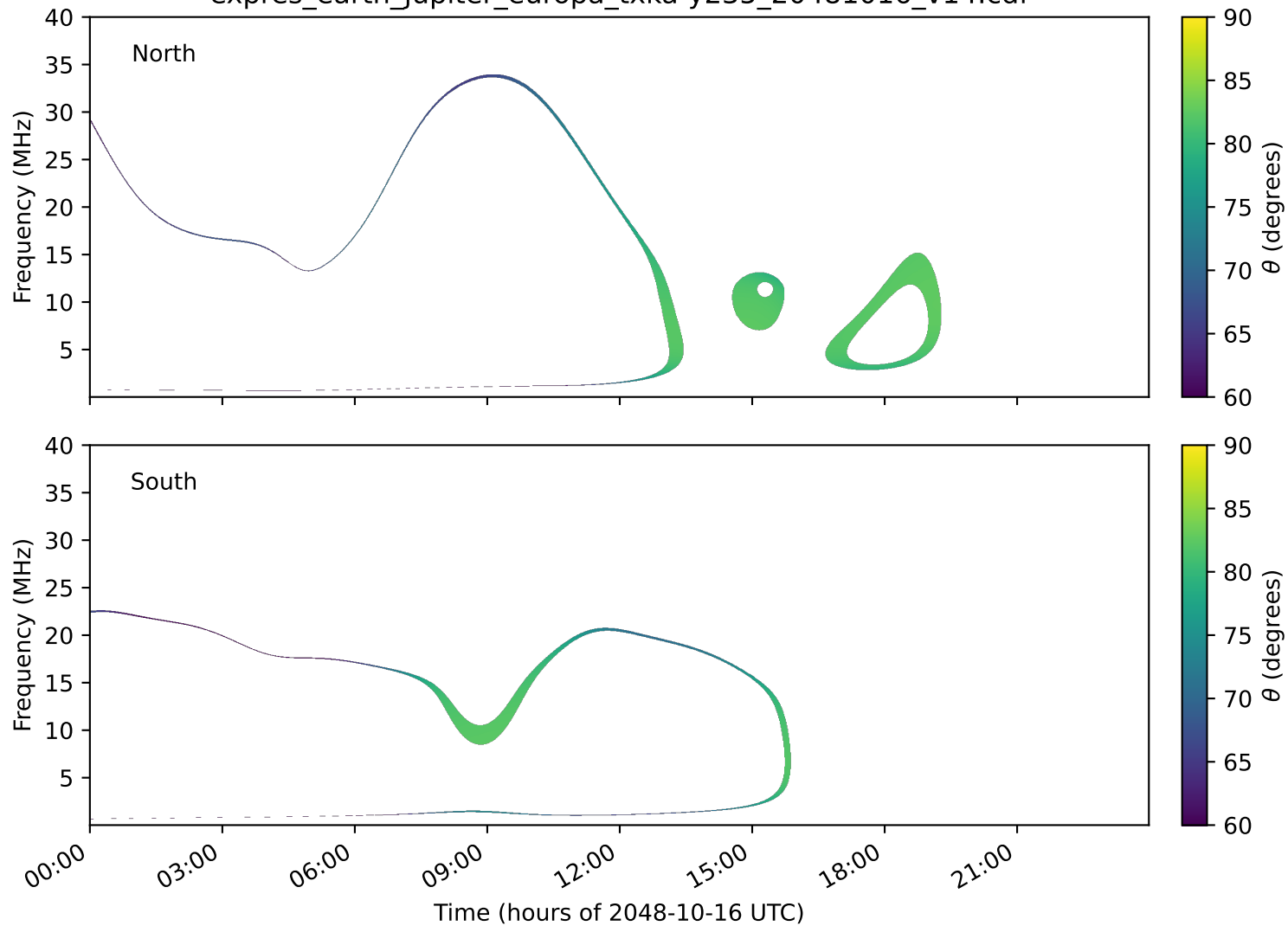
expres_earth_jupiter_europa_txka-y235_20481016_v14.cdf
