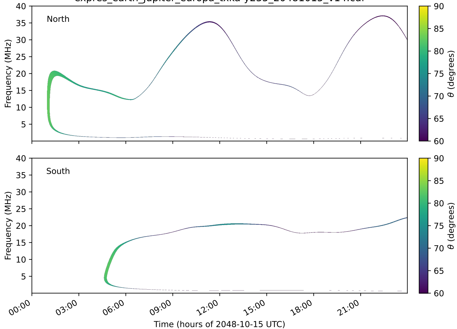
expres_earth_jupiter_europa_txka-y235_20481015_v14.cdf
