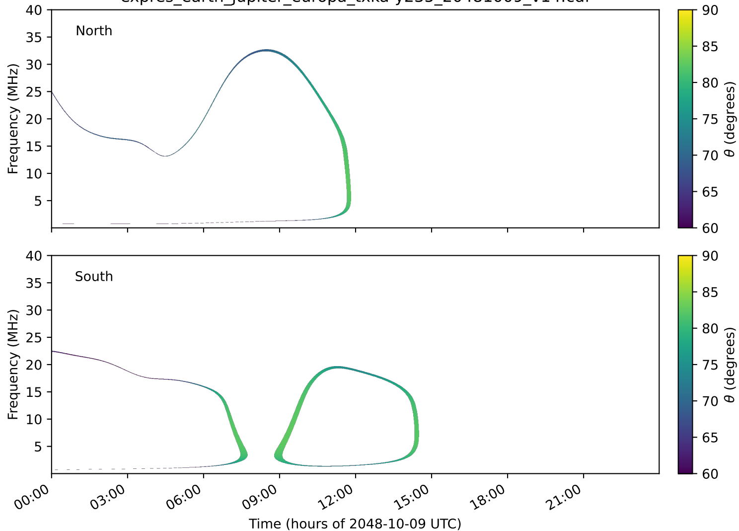
expres_earth_jupiter_europa_txka-y235_20481009_v14.cdf
