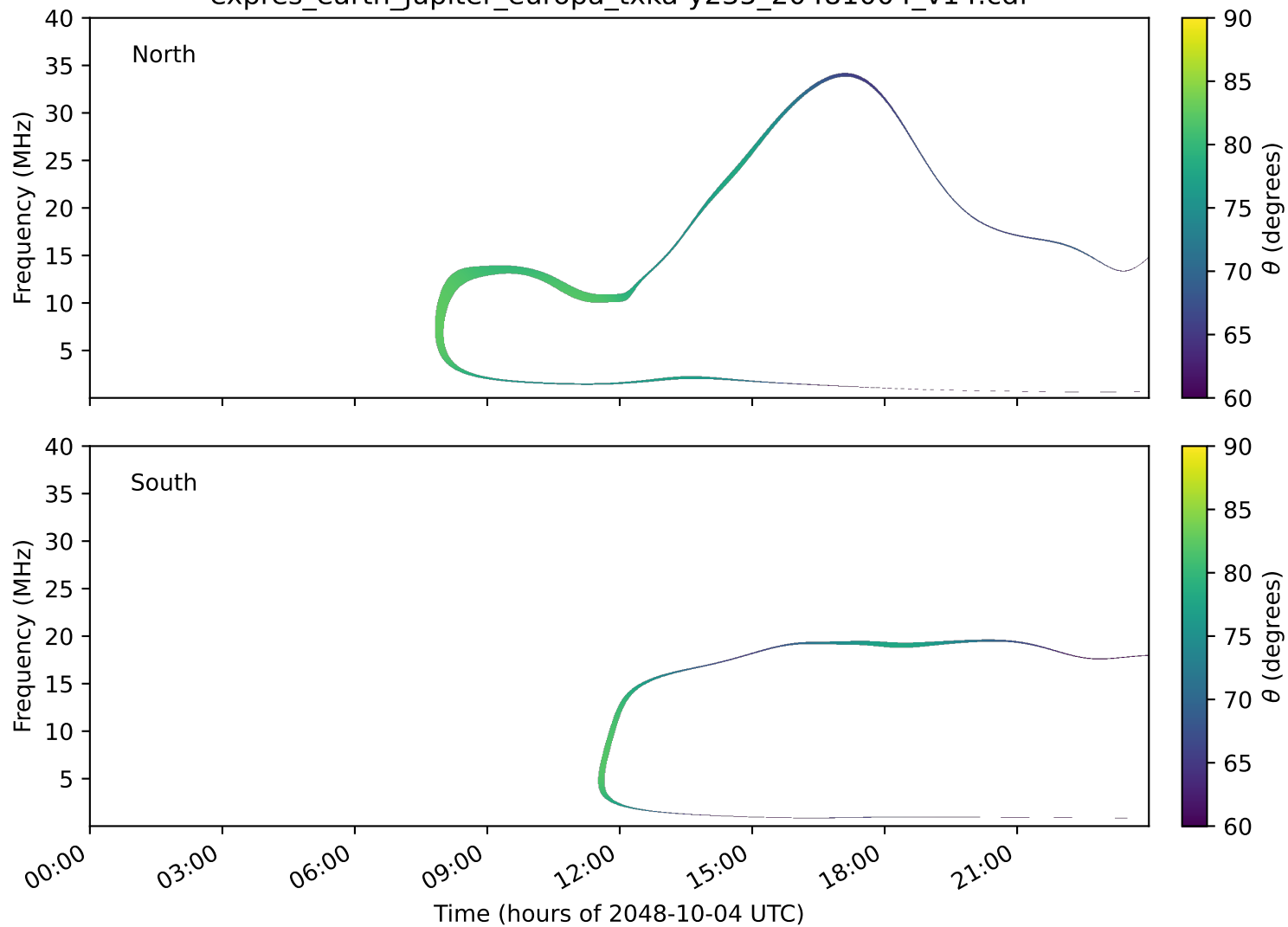
expres_earth_jupiter_europa_txka-y235_20481004_v14.cdf
