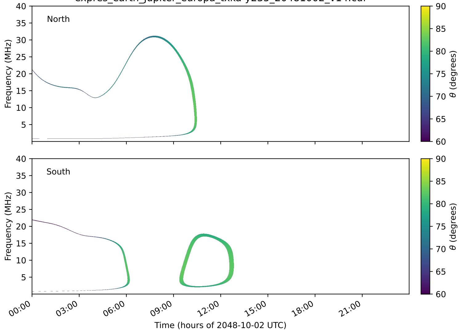
expres_earth_jupiter_europa_txka-y235_20481002_v14.cdf
