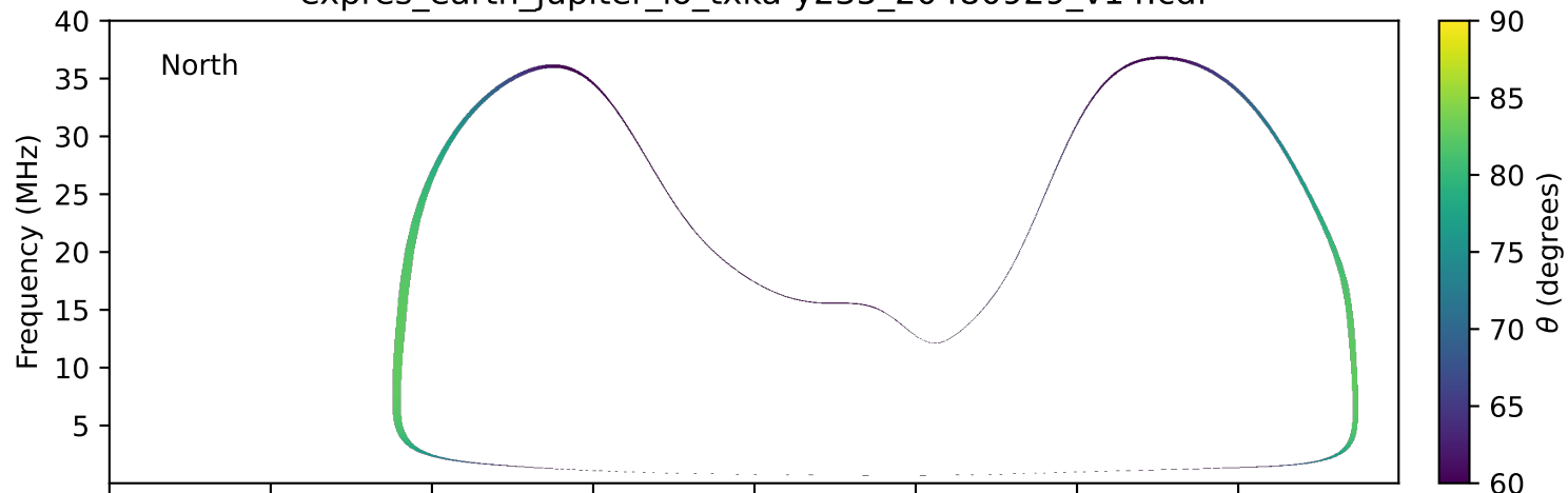
expres_earth_jupiter_io_txka-y235_20480929_v14.cdf
