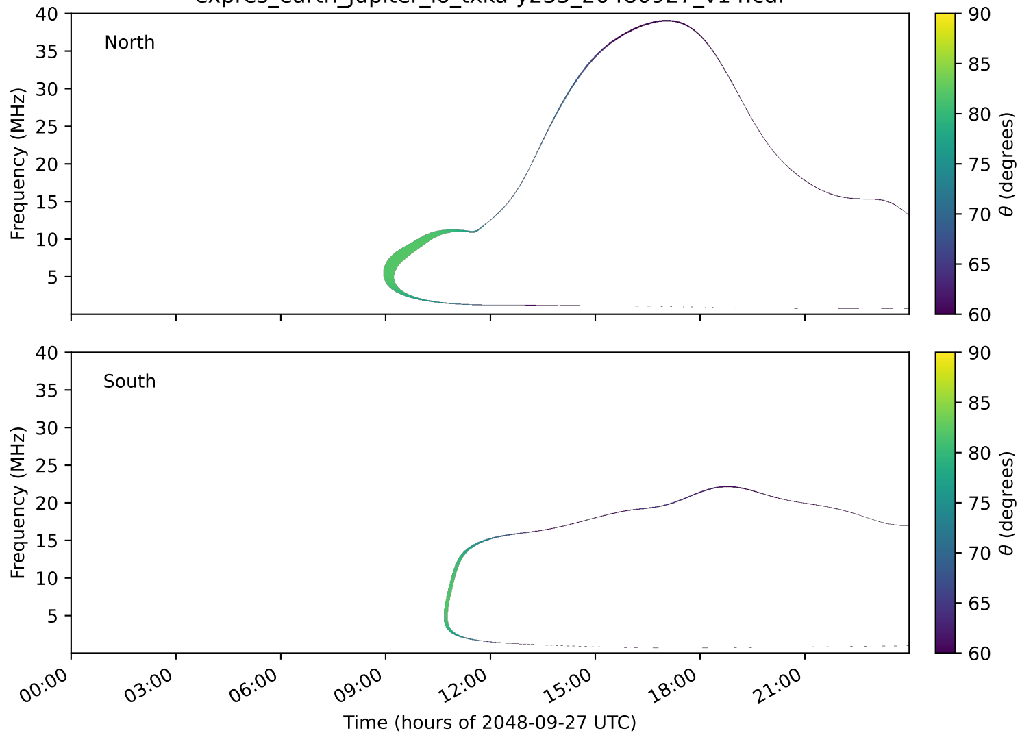
expres_earth_jupiter_io_txka-y235_20480927_v14.cdf
