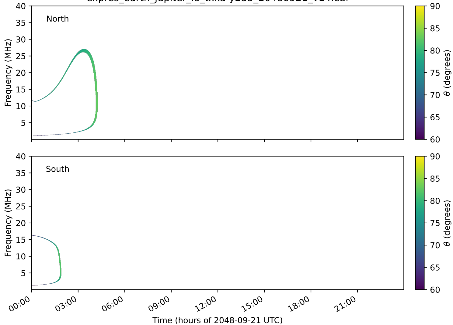
expres_earth_jupiter_io_txka-y235_20480921_v14.cdf
