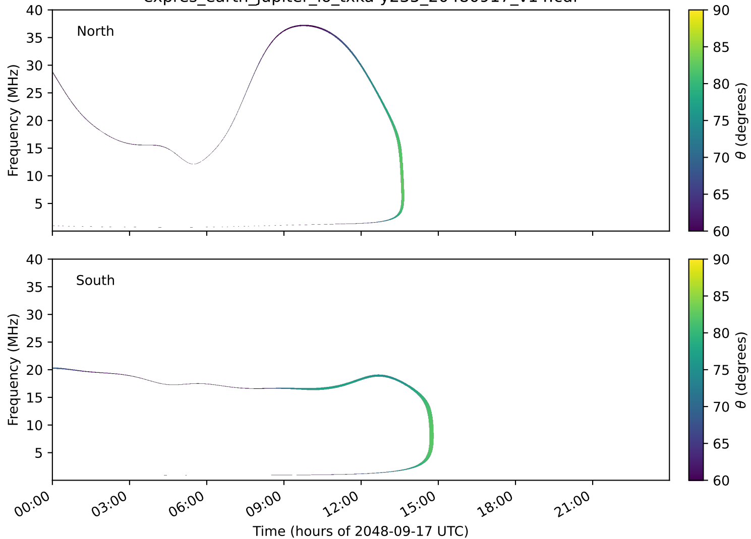
expres_earth_jupiter_io_txka-y235_20480917_v14.cdf
