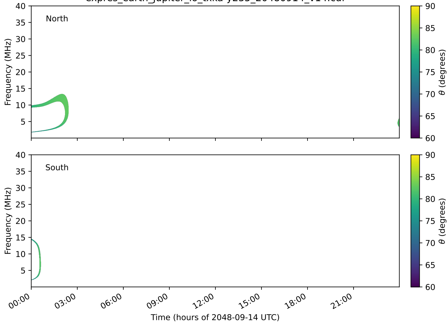
expres_earth_jupiter_io_txka-y235_20480914_v14.cdf
