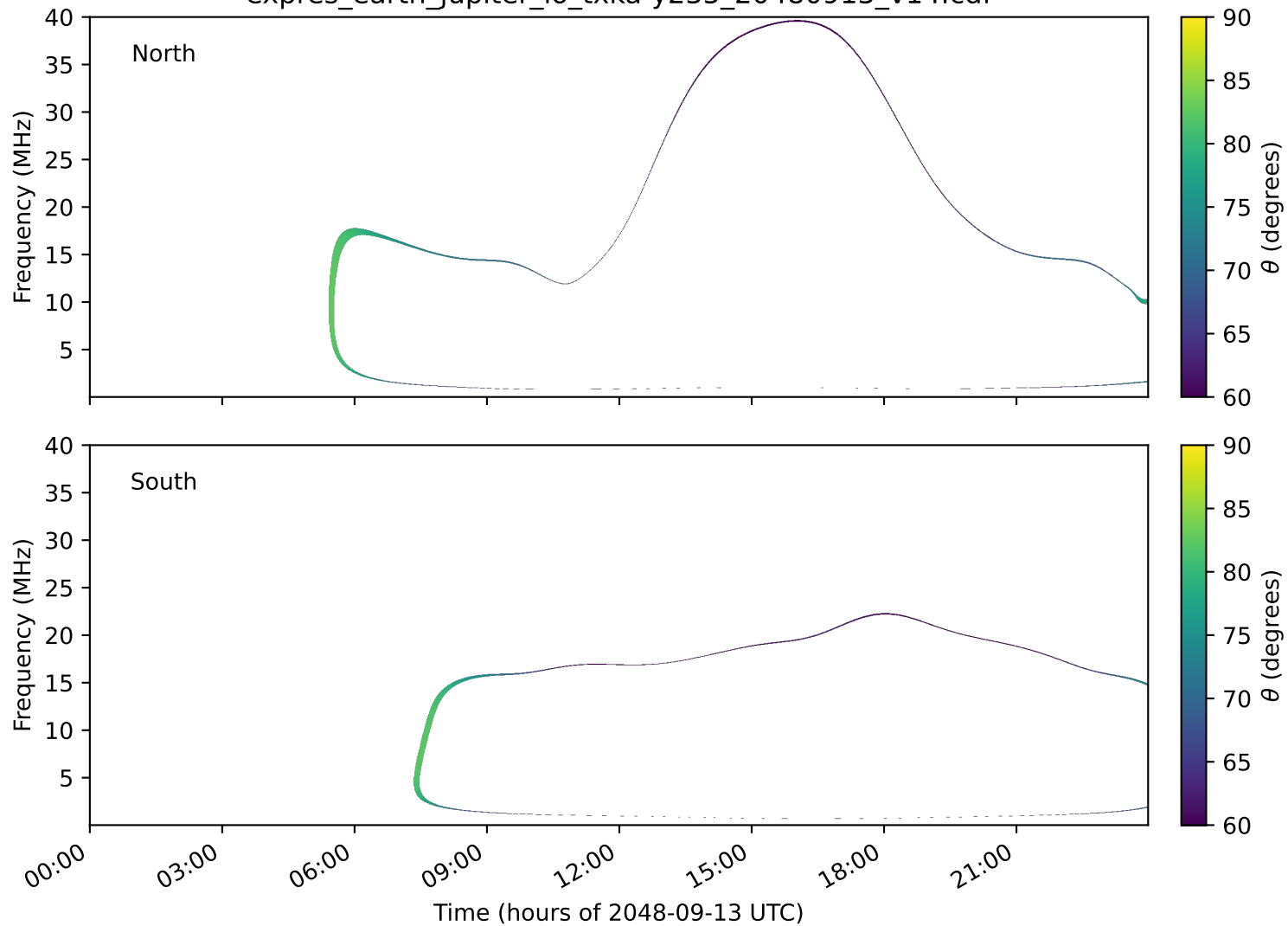
expres_earth_jupiter_io_txka-y235_20480913_v14.cdf
