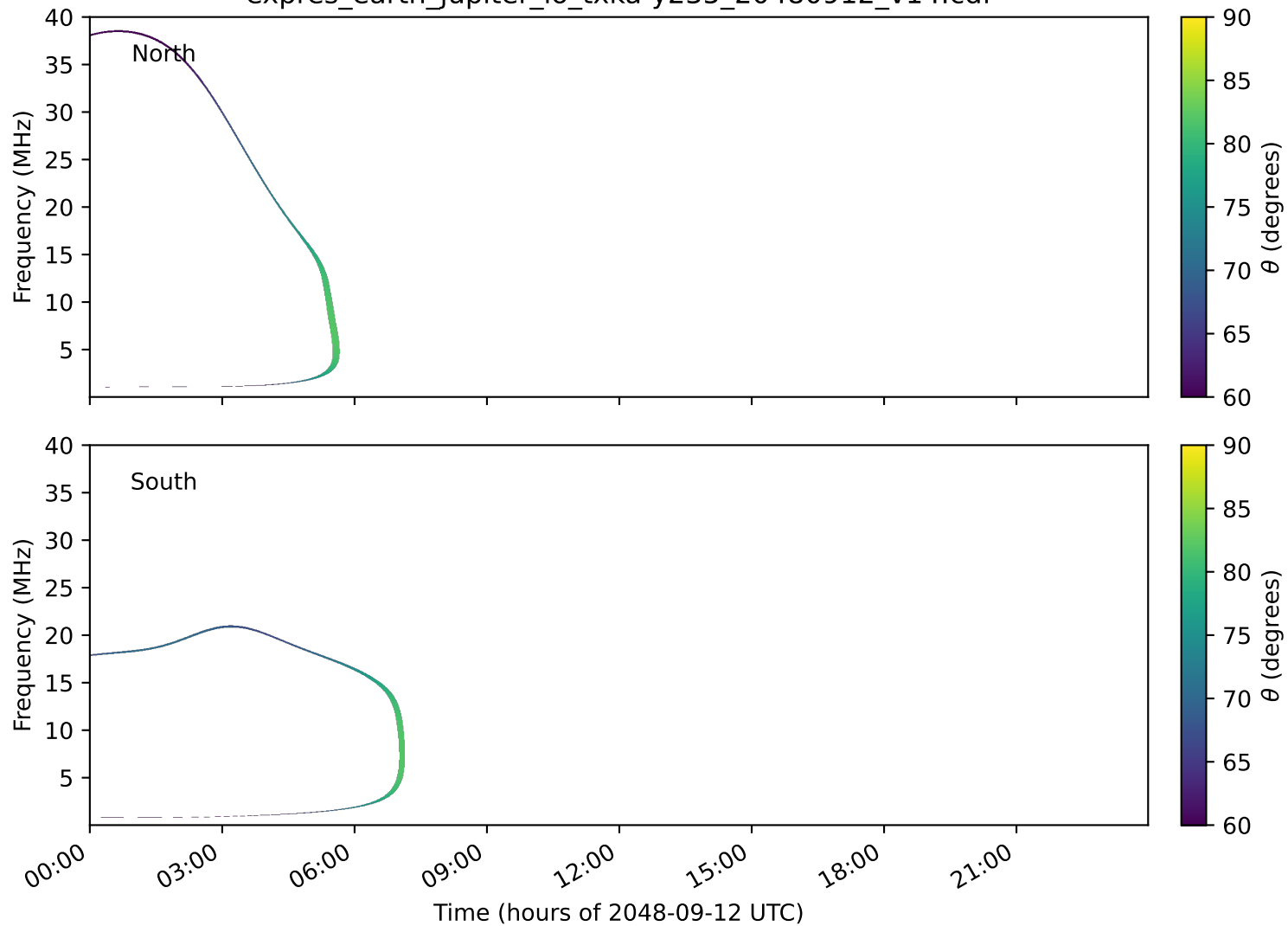
expres_earth_jupiter_io_txka-y235_20480912_v14.cdf
