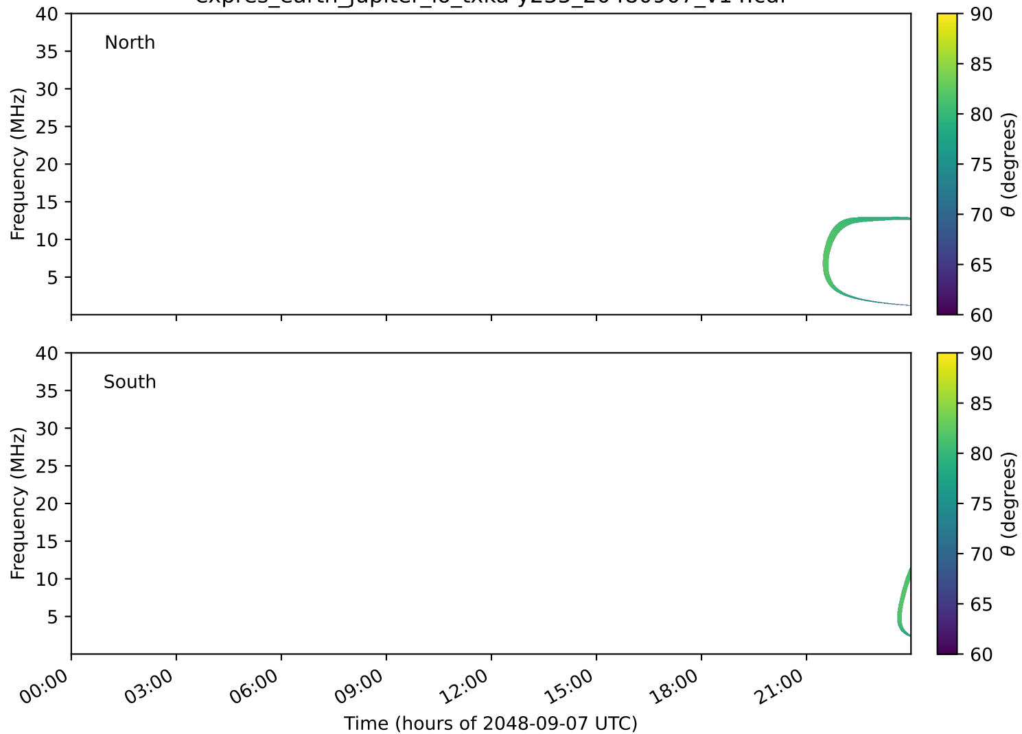
expres_earth_jupiter_io_txka-y235_20480907_v14.cdf
