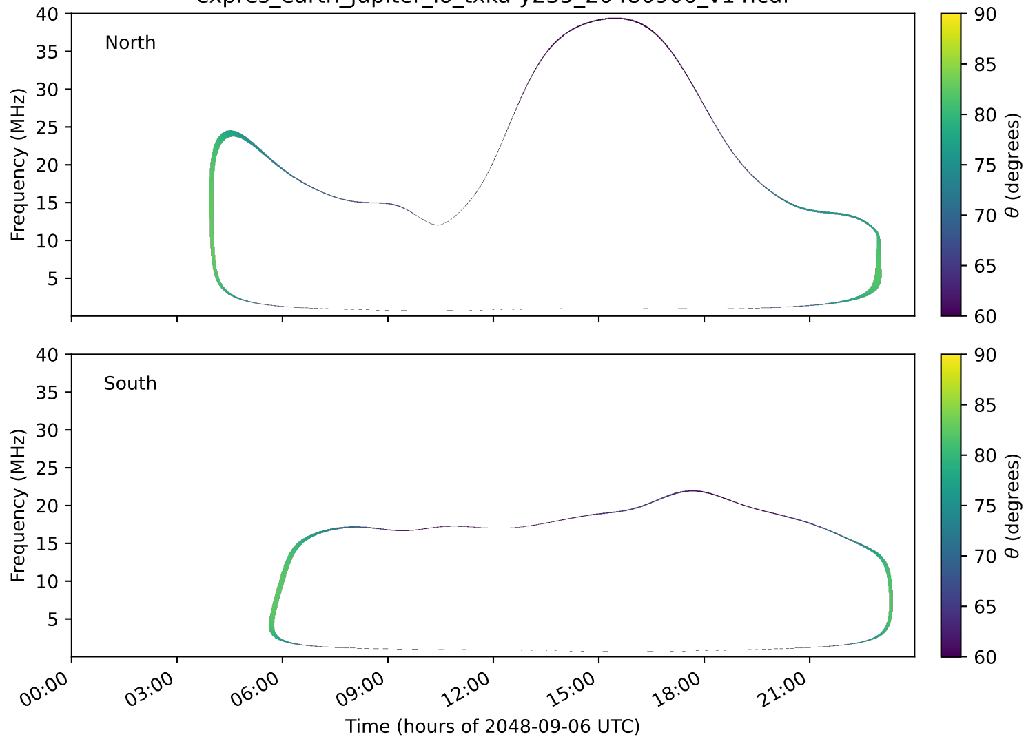
expres_earth_jupiter_io_txka-y235_20480906_v14.cdf
