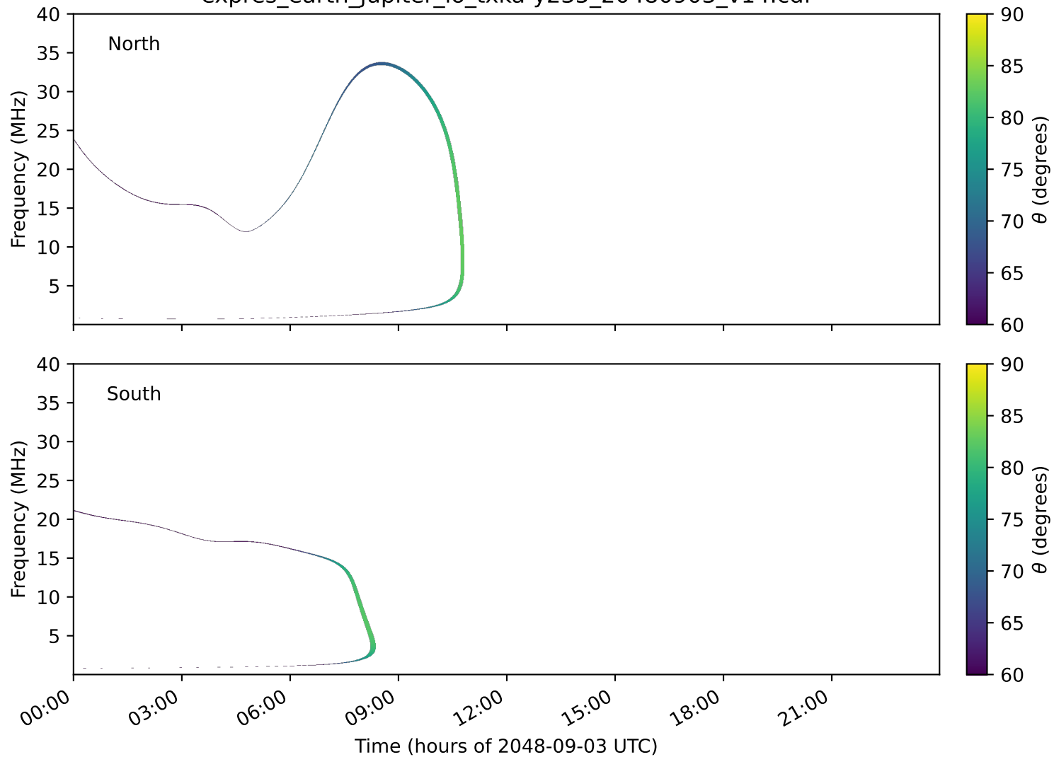
expres_earth_jupiter_io_txka-y235_20480903_v14.cdf
