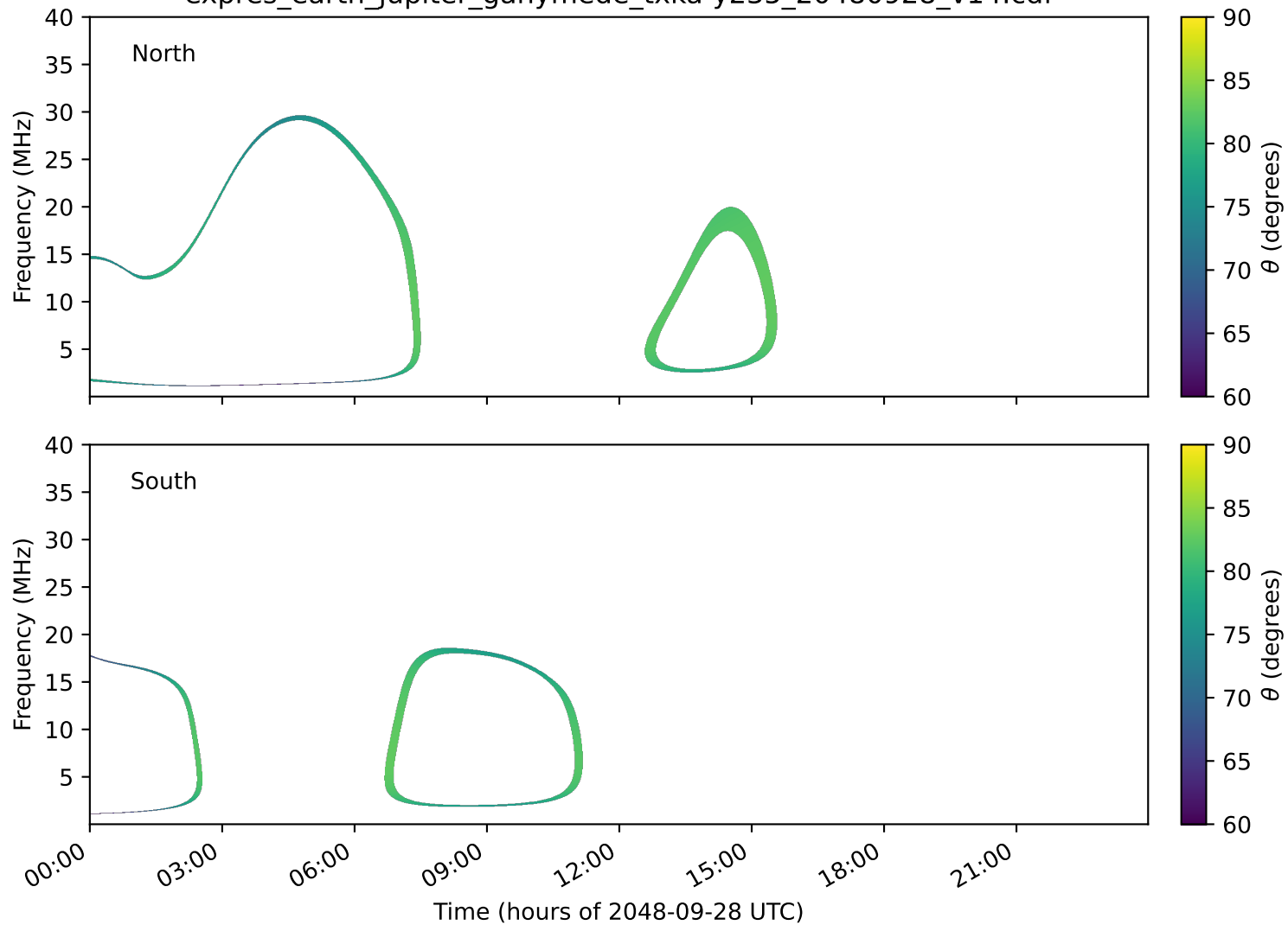
expres_earth_jupiter_ganymede_txka-y235_20480928_v14.cdf
