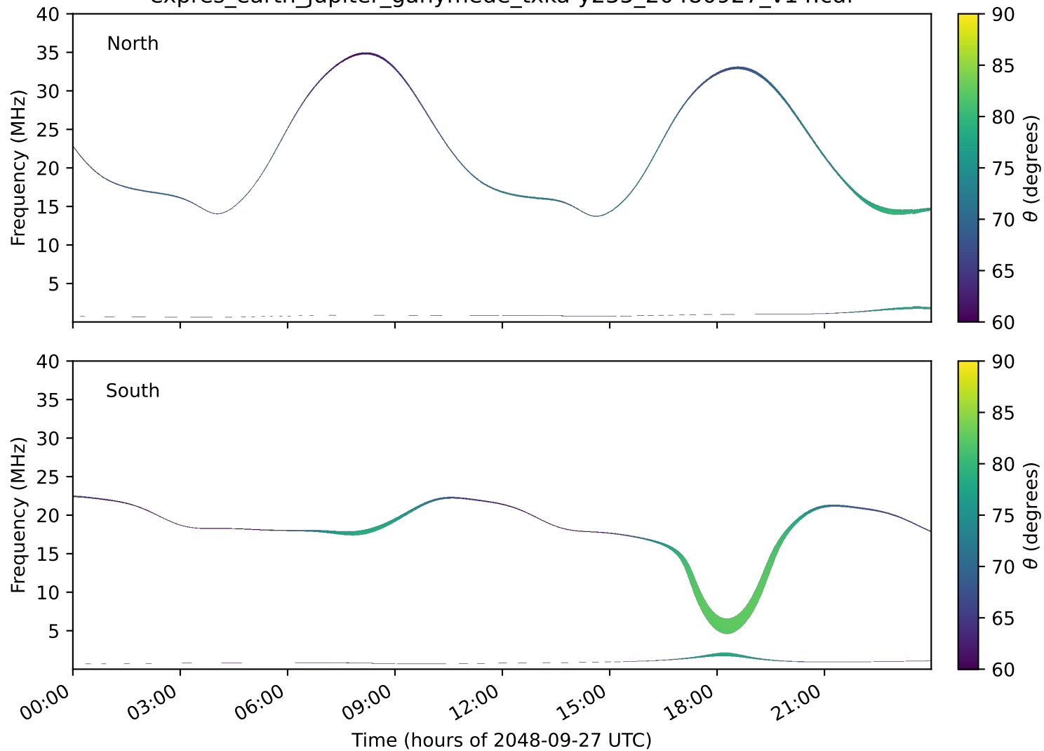
expres_earth_jupiter_ganymede_txka-y235_20480927_v14.cdf
