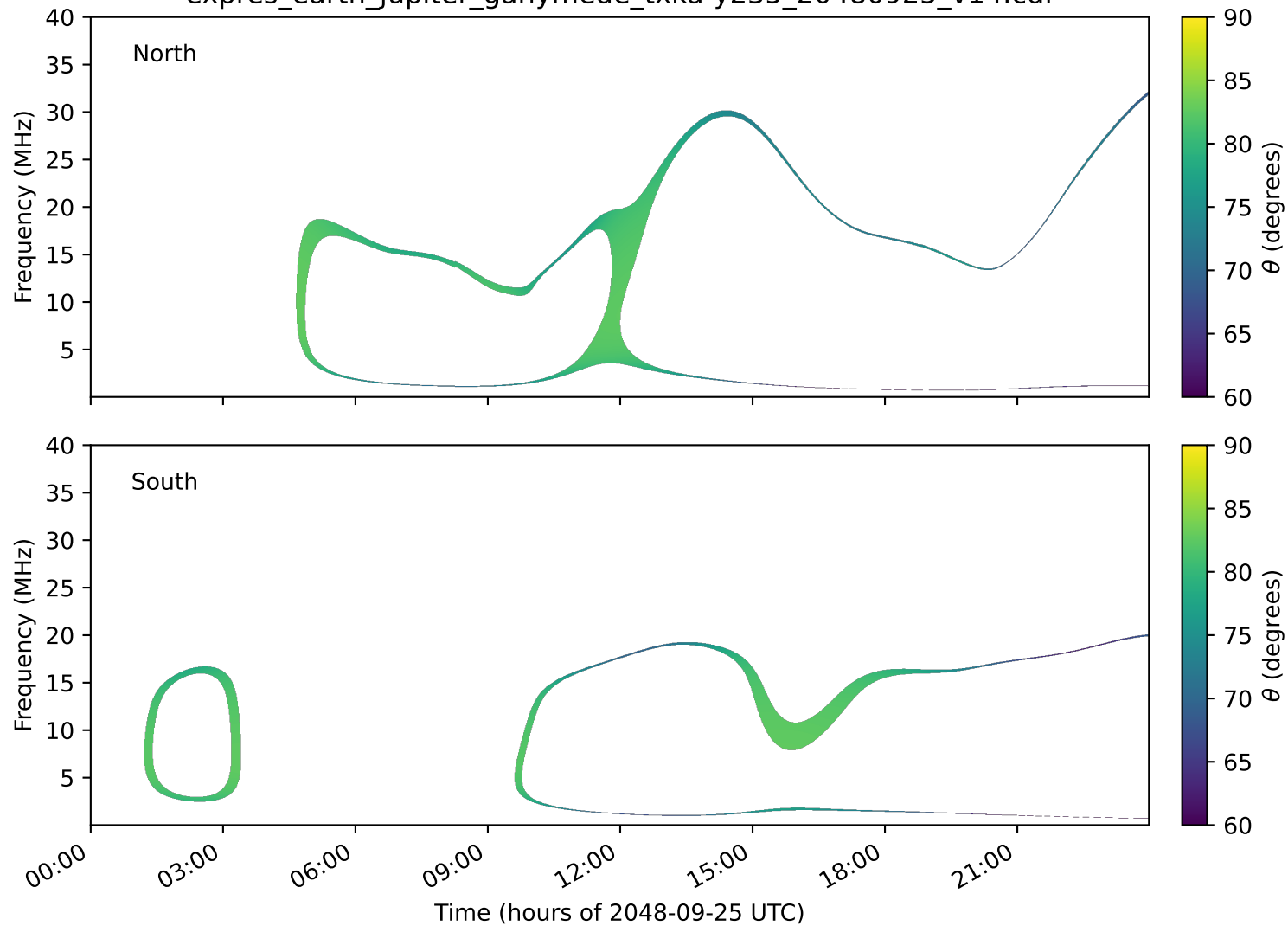
expres_earth_jupiter_ganymede_txka-y235_20480925_v14.cdf
