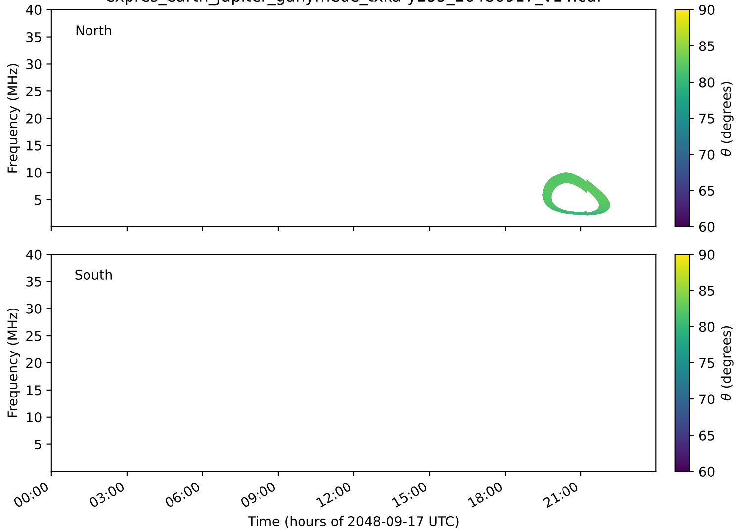
expres_earth_jupiter_ganymede_txka-y235_20480917_v14.cdf
