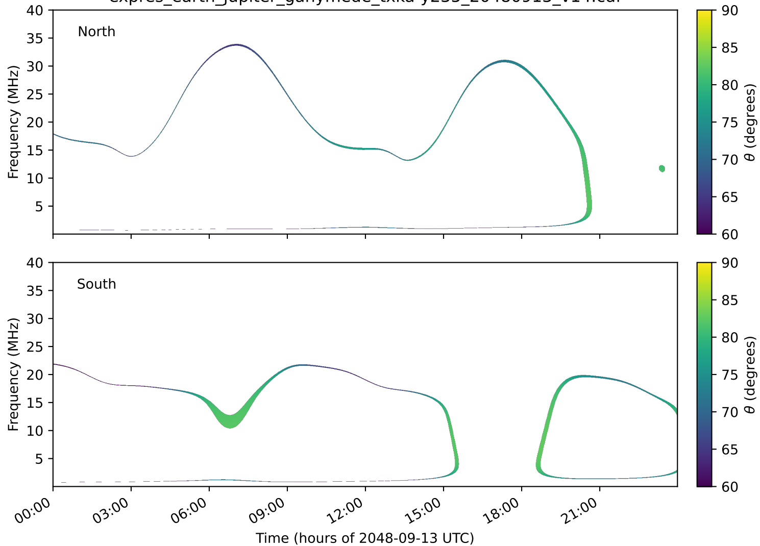
expres_earth_jupiter_ganymede_txka-y235_20480913_v14.cdf
