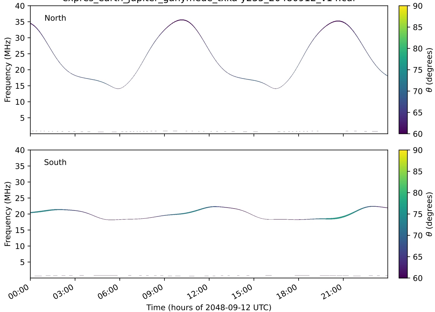
expres_earth_jupiter_ganymede_txka-y235_20480912_v14.cdf
