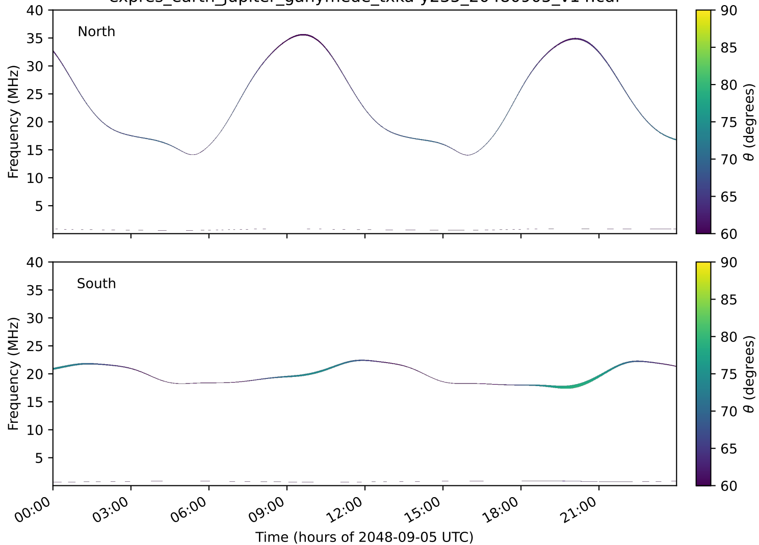
expres_earth_jupiter_ganymede_txka-y235_20480905_v14.cdf
