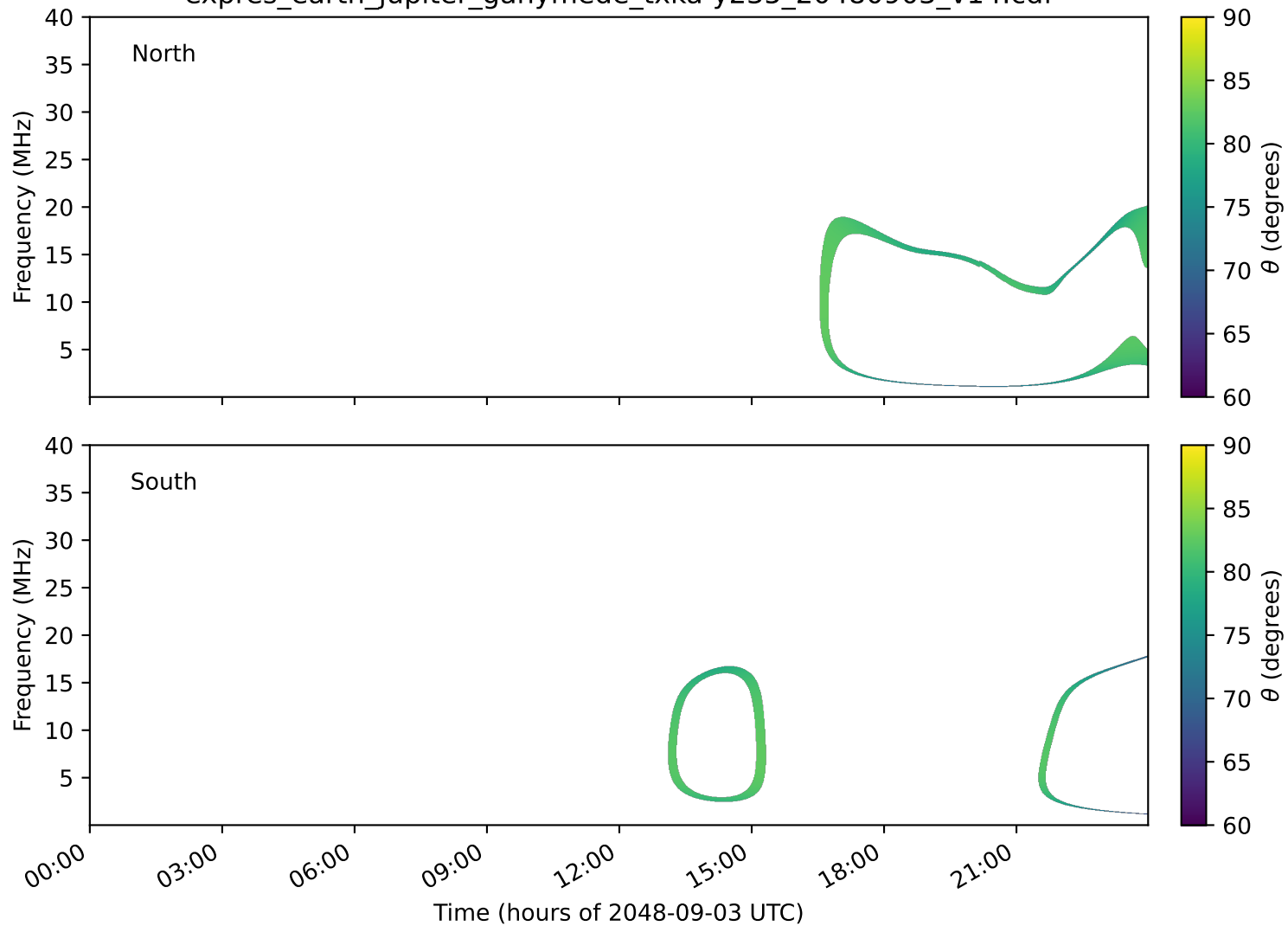
expres_earth_jupiter_ganymede_txka-y235_20480903_v14.cdf
