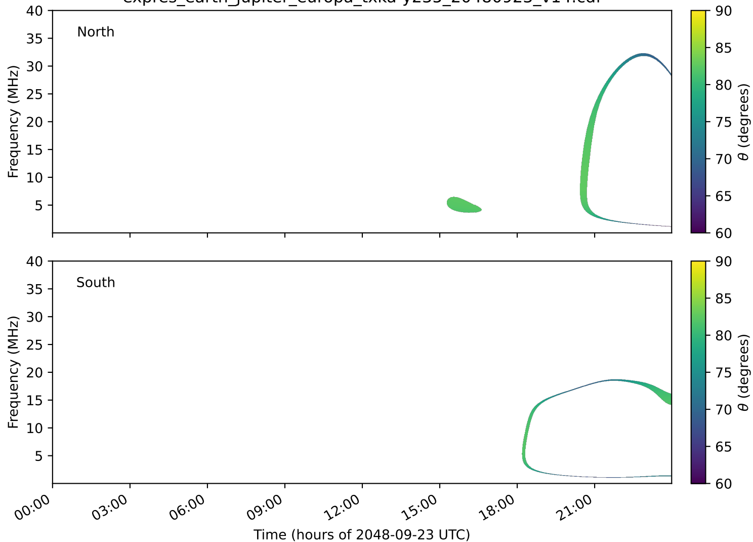
expres_earth_jupiter_europa_txka-y235_20480923_v14.cdf
