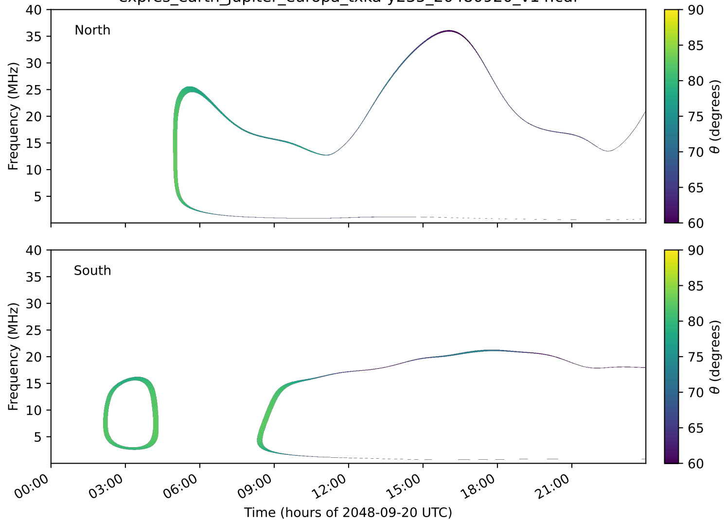
expres_earth_jupiter_europa_txka-y235_20480920_v14.cdf
