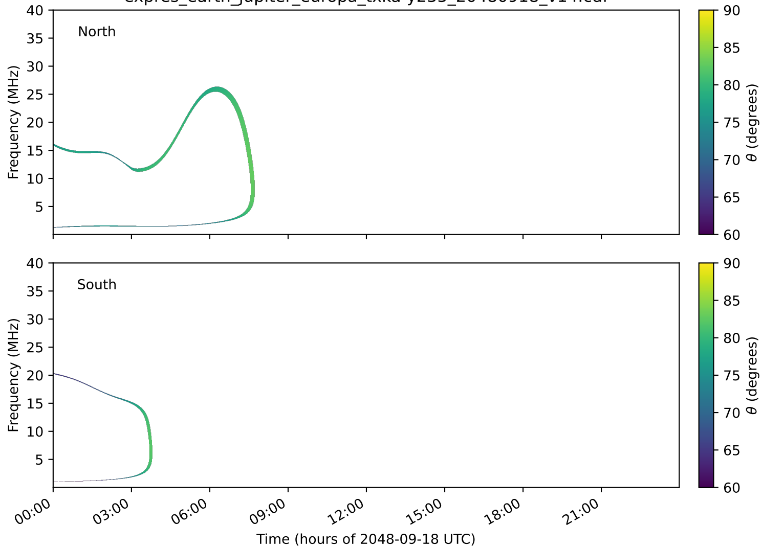
expres_earth_jupiter_europa_txka-y235_20480918_v14.cdf
