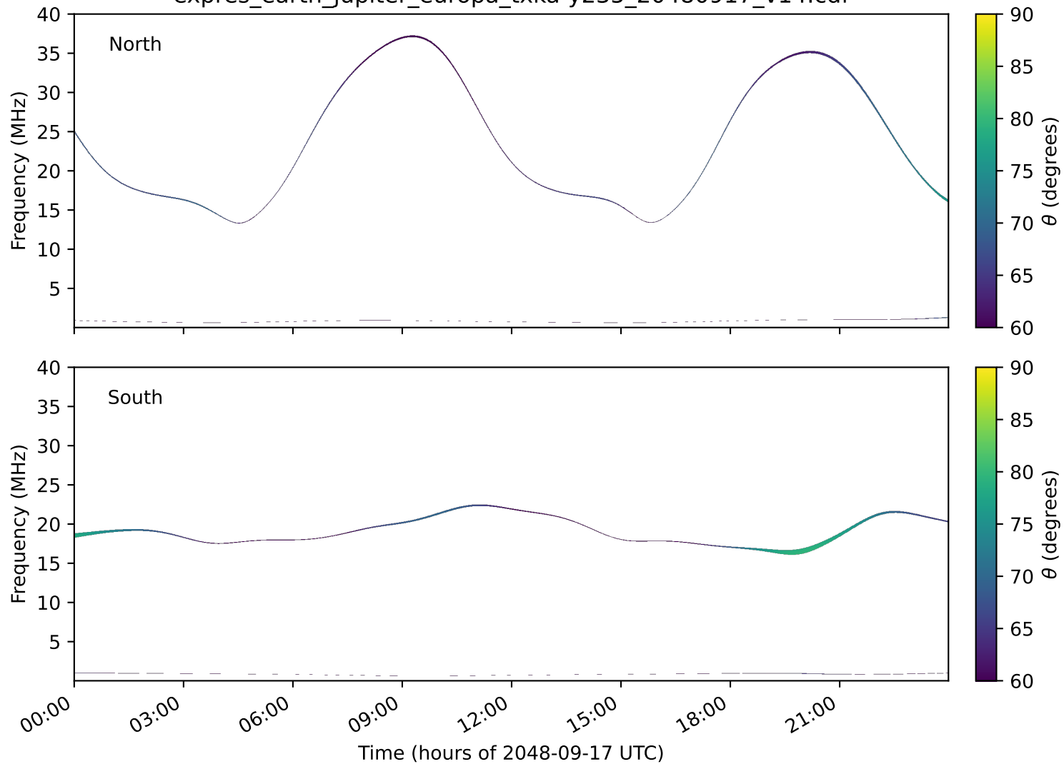
expres_earth_jupiter_europa_txka-y235_20480917_v14.cdf
