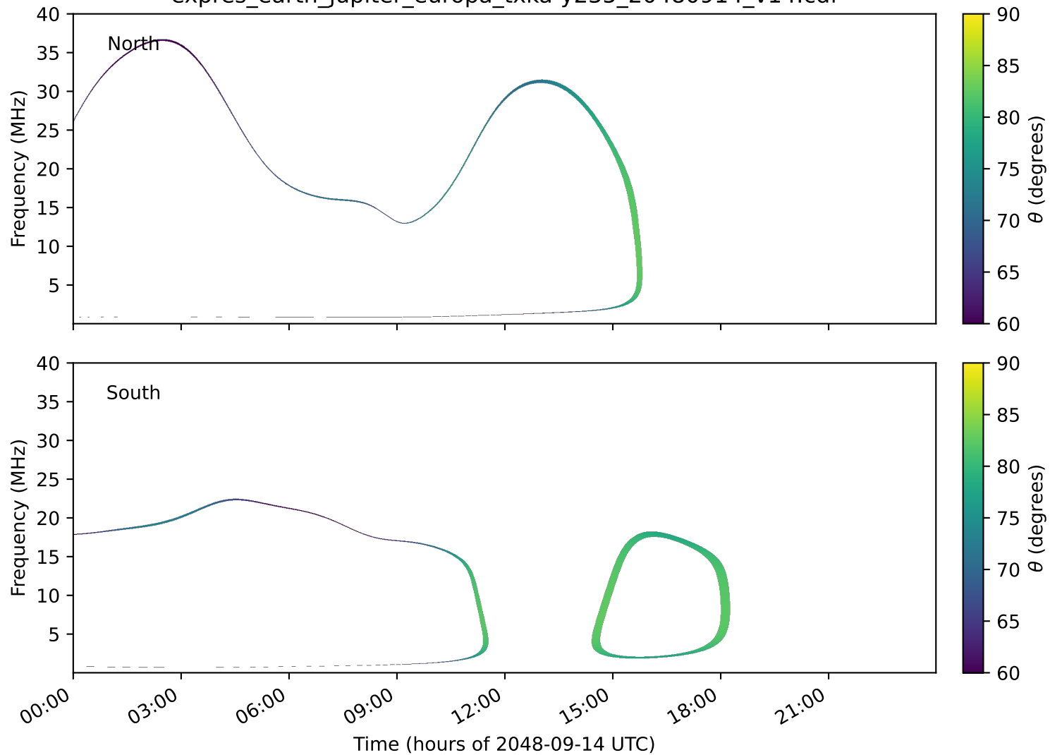
expres_earth_jupiter_europa_txka-y235_20480914_v14.cdf
