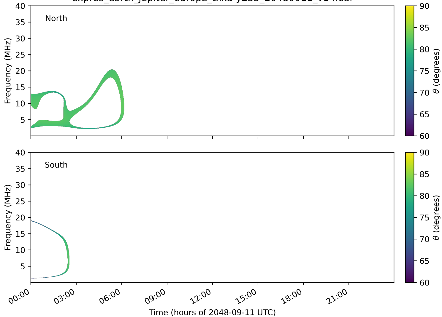
expres_earth_jupiter_europa_txka-y235_20480911_v14.cdf
