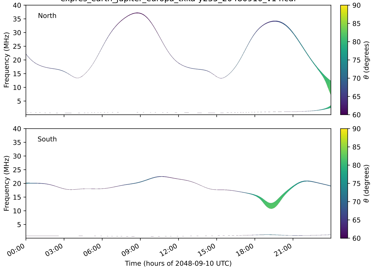
expres_earth_jupiter_europa_txka-y235_20480910_v14.cdf
